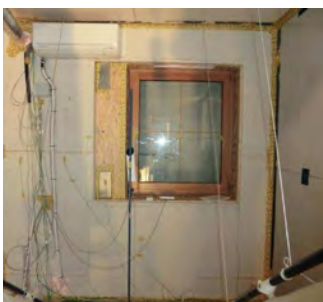
Inside view of wall with integrated micro heat pump (Project iNSPiRe)
