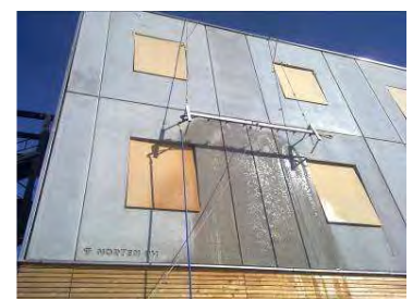
Water tightness analysis of the prefabricated concrete façade element
