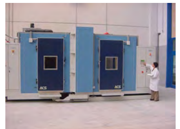
Guarded hot box for opaque walls (according to EN ISO 8990)
