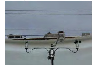
ILARGI air temperature, velocity and direction in the height of the roof.
