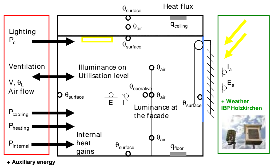
Measurement point overview in test rooms
