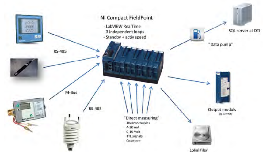
Figure 5. The data acquisition system in EnergyFlexLab.
