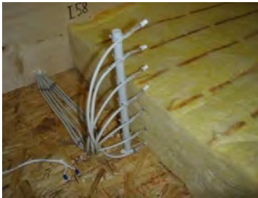
Combined heat/moisture sensors in roof assembly
