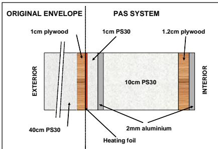
Schematic drawing of the PAS system
