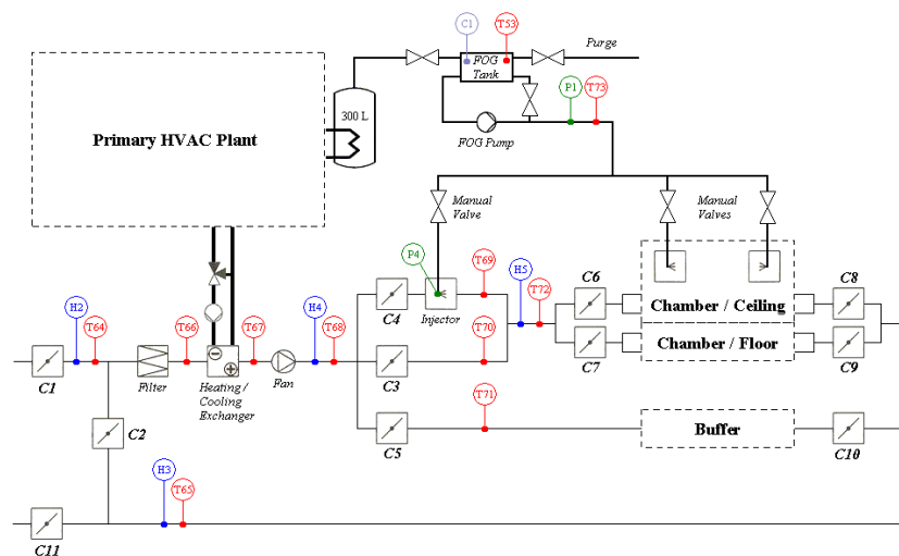
Overview of sensors installed on the Air-Handling Unit
